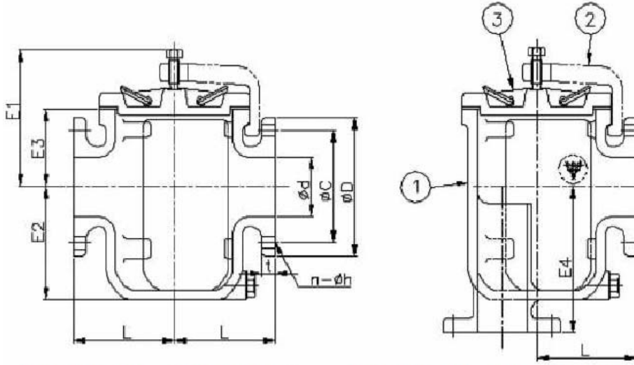
SERIES F 7203 – S type Mud Box
